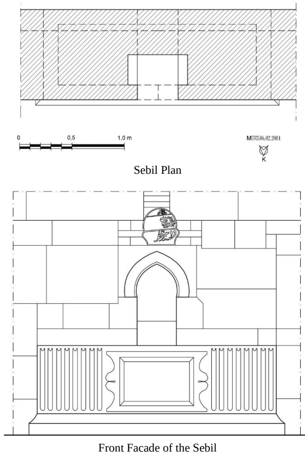
Figure 10. Plan and facade view of the Sebil at Meram Hoca Ahmet Fakih Complex (M. Mutlu)
