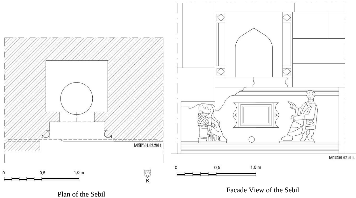
Figure 8. Plan and facade view of the sebil of Beyşehir Eşrefoğlu Mosque Complex (M. Mutlu)
