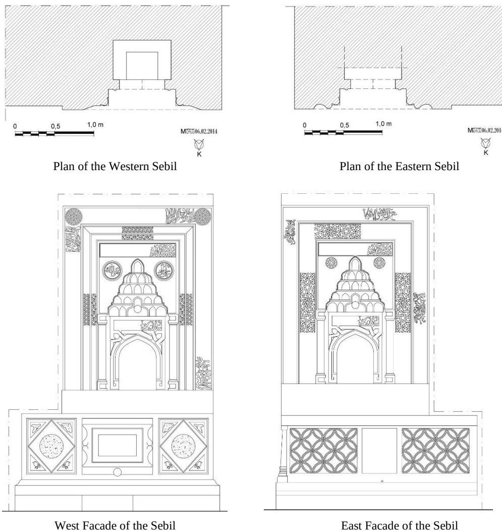
Figure 5. Plans and Facade Views of the Sahip Ata Complex Sebils (M. Mutlu)
